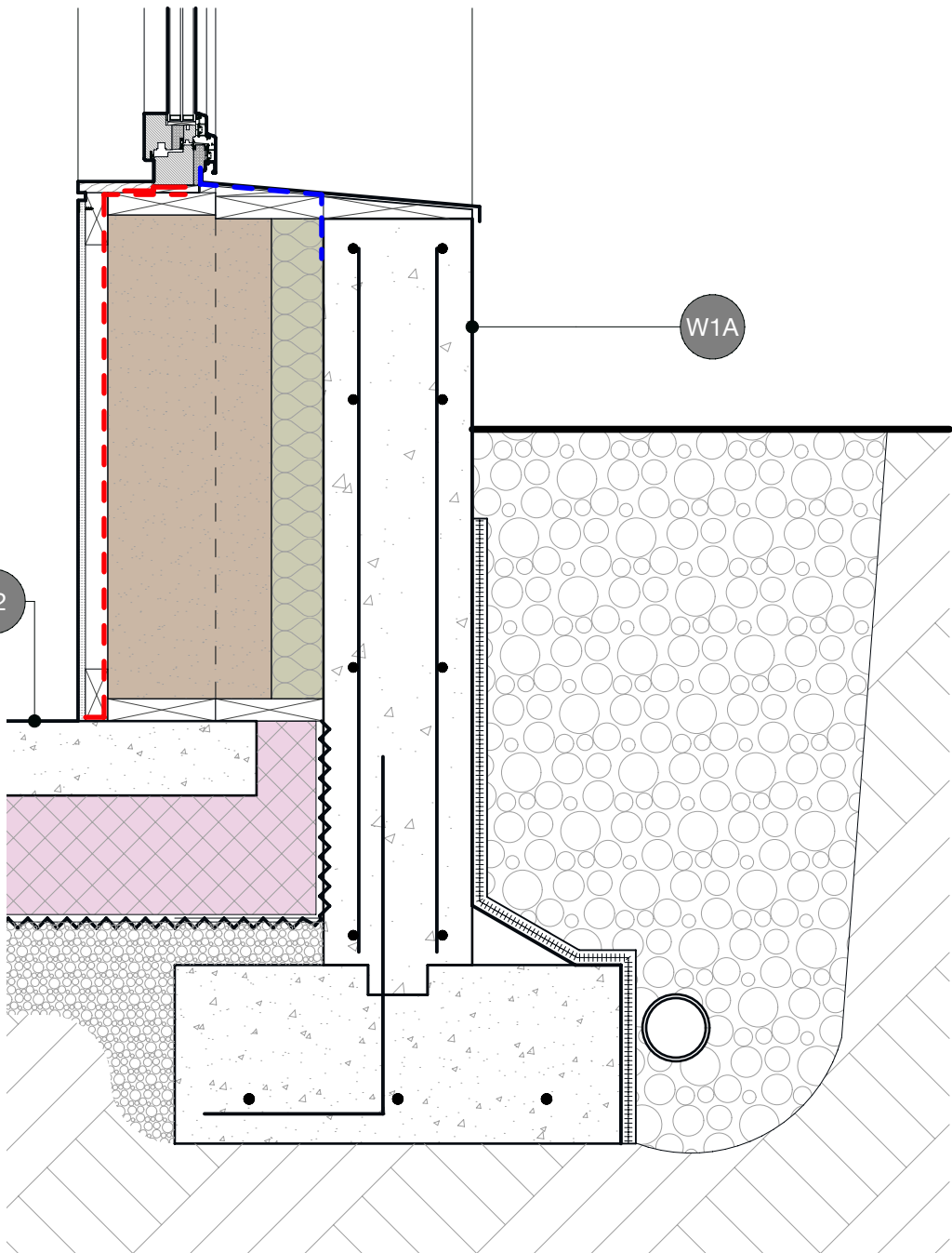
TYP. WALL SECTION
