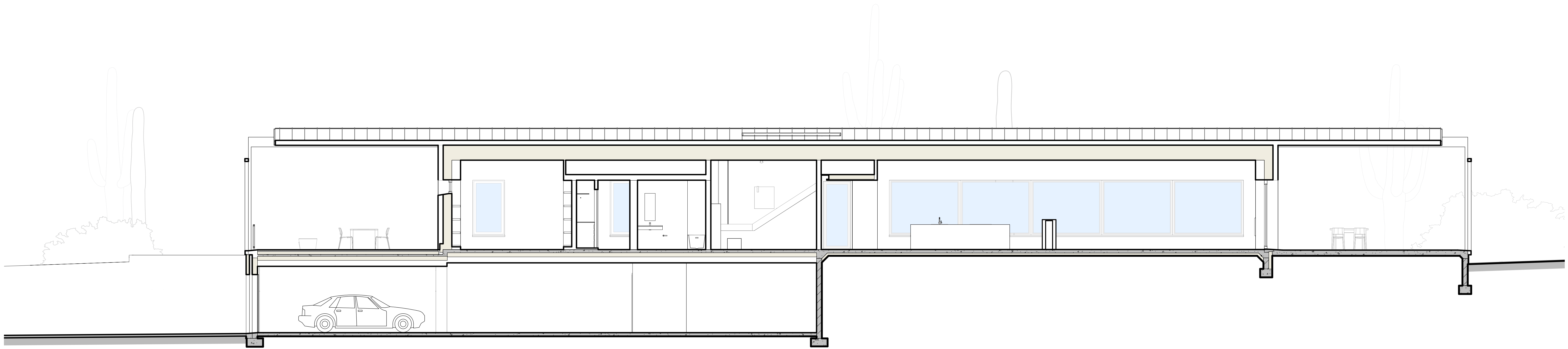
Section A - Looking North
